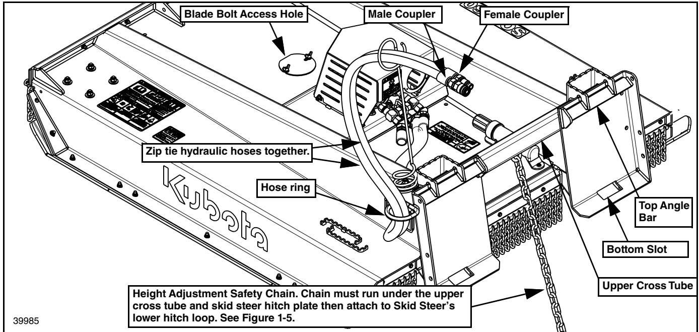
Skid Steer Hook-Up Figure 1-4
