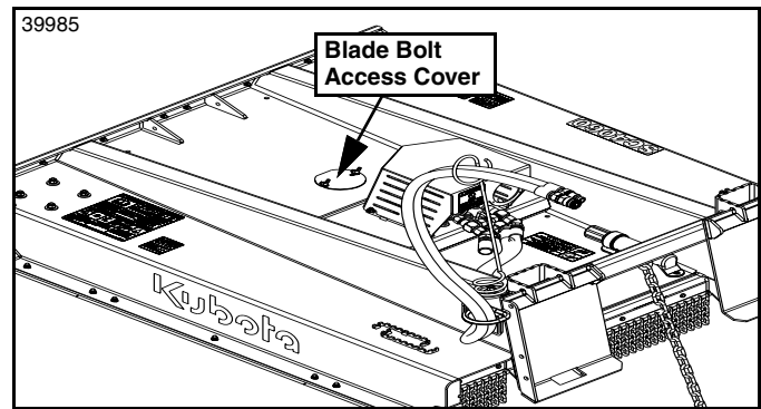
Blade Bolt Access Cover Location Figure 5-1
