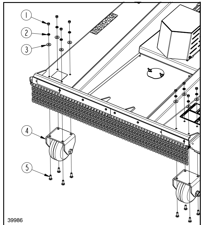
Front Roller Wheel Assembly Figure 1-7
