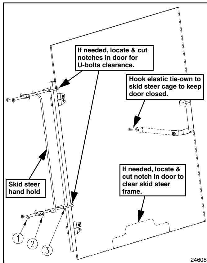
Polycarbonate Protective Door Assembly Figure 1-10
