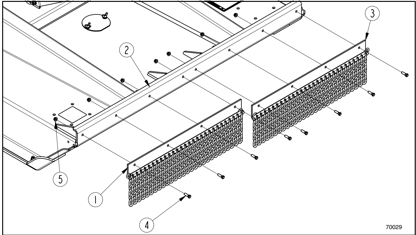
SC4060 &amp; SC4072 Front Chain Guard Assembly
