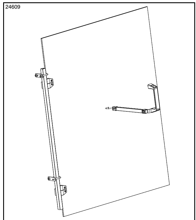
Polycarbonate Protective Door Figure 4-6
