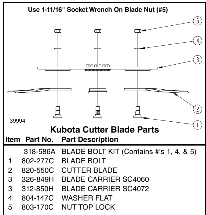
Cutter Blade Assembly Figure 5-2
