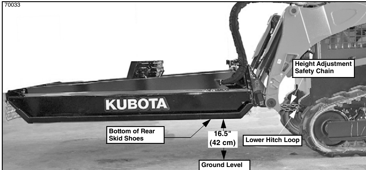
Nominal Cutting Height (SVL shown) Figure 2-1
