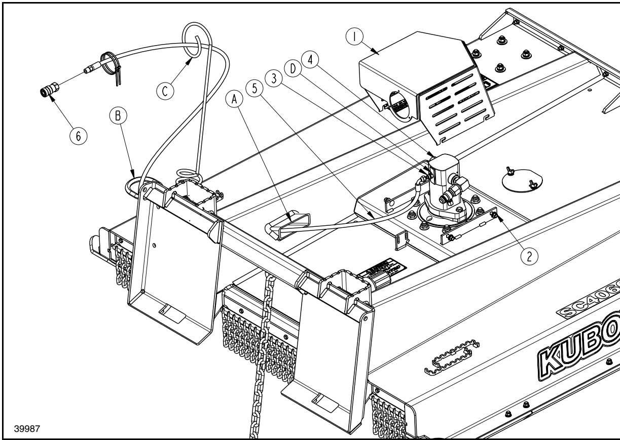
Case Drain Assembly Figure 1-8
