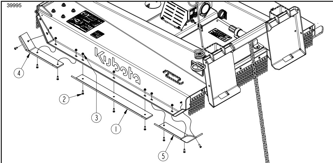
Skid Shoe Replacement Figure 5-3
