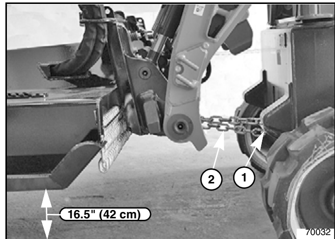
SC40 Height Adjustment (SVL Shown) Figure 2-2
