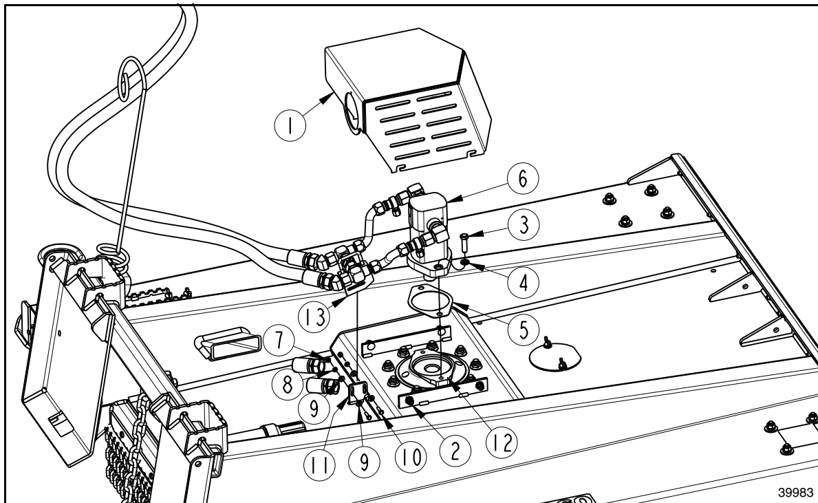
SC4060 &amp; SC4072 Motor and Hose Assembly
