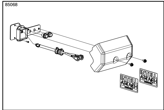
Receiver/Cover Assembly Figure 4-8
