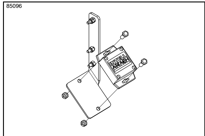
Tag/Bracket Assembly Figure 4-9
