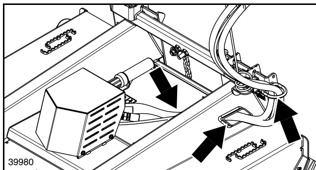
SC4060 &amp; SC4072 Hose Routing
