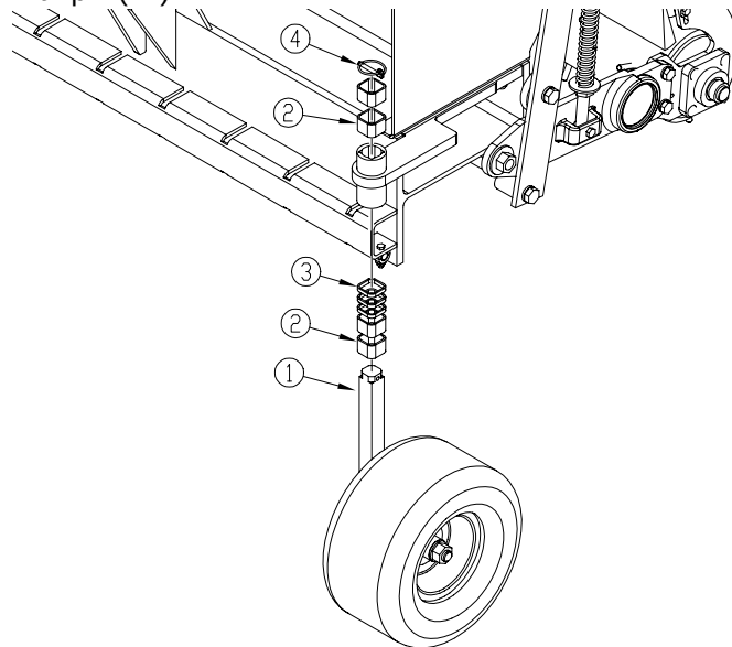
Shank Working Depth Figure 3-5
