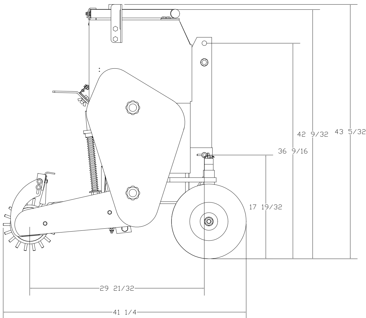
SPS3072 Specification Drawing Figure 7-1
