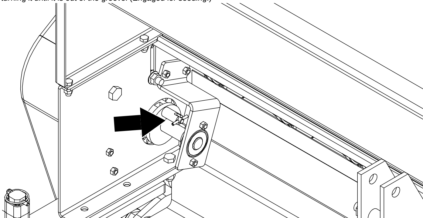
Clutch Engagement Figure 3-6
