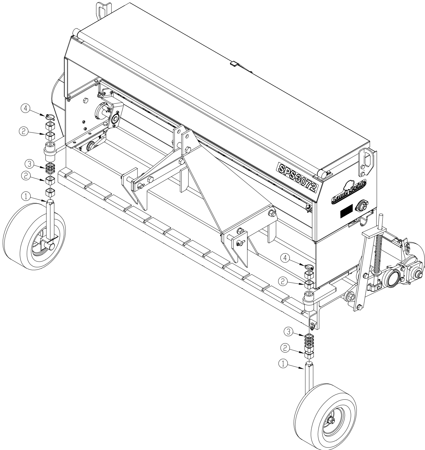
Dealer Gauge Wheel Assembly Figure 1-1
