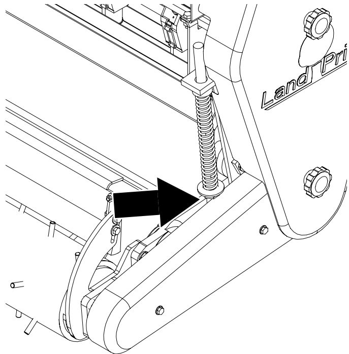
Down Pressure Adjustment Figure 3-3
