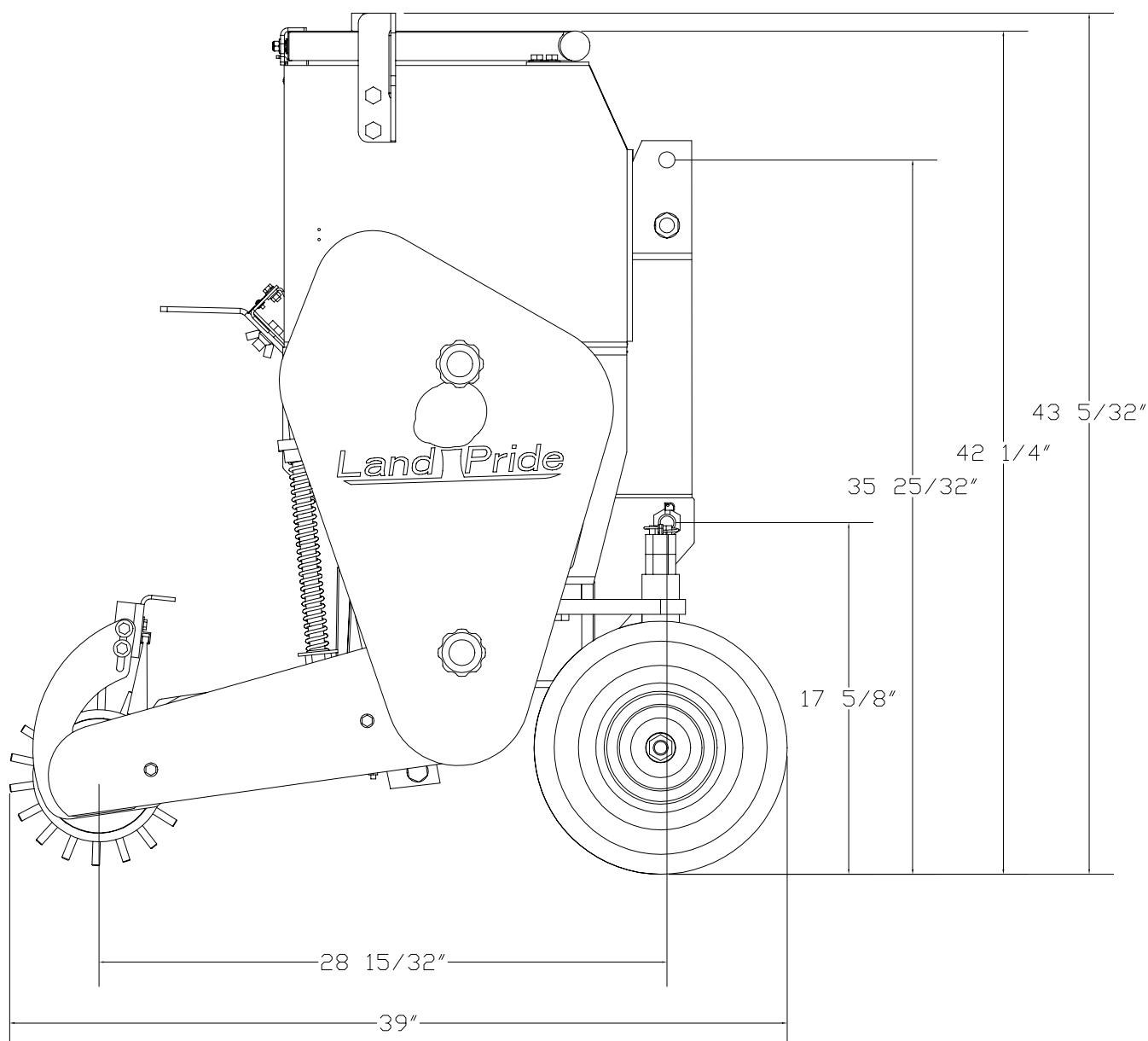
SPS2048 Specification Drawing Figure 7-2
